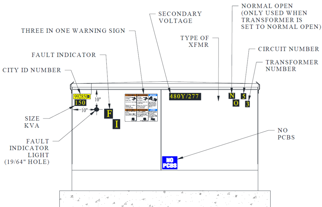
3 PHASE PAD MOUNTED TRANSFORMER LID/DOOR SIDE
