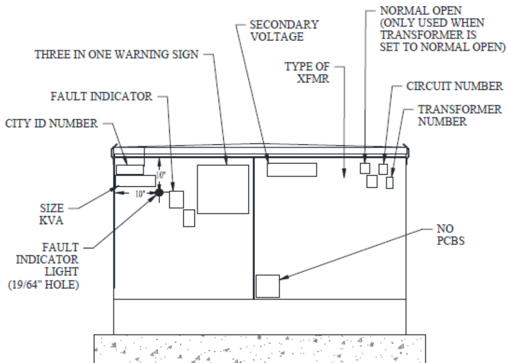
3 PHASE PAD MOUNTED TRANSFORMER LID/DOOR SIDE
